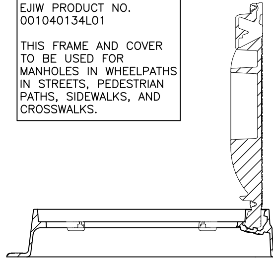
SAFETY LOCK @ 90°
